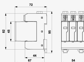
Product dimensions
